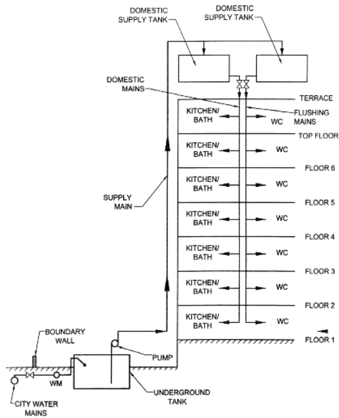
Figure 8 Overhead Tank Distribution
