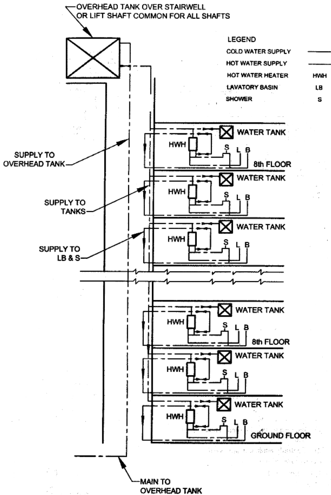
Figure 11 Installation For 8 – Storeyed Building with Individual Water Tanks
