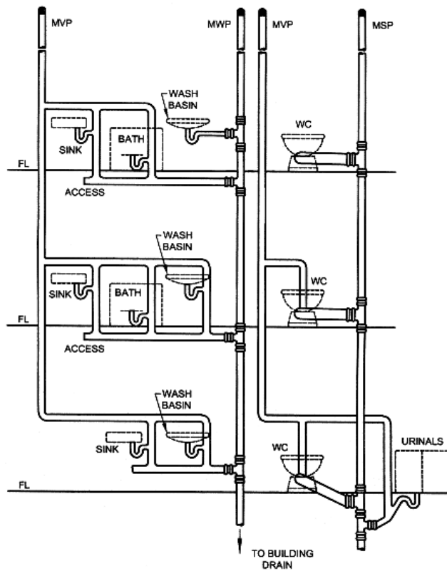
Figure 4 Diagram Of Two-Pipe System
