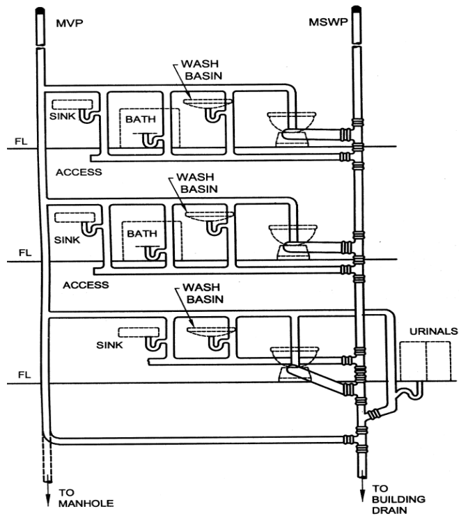
Figure 3 Diagram Of One-Pipe System
