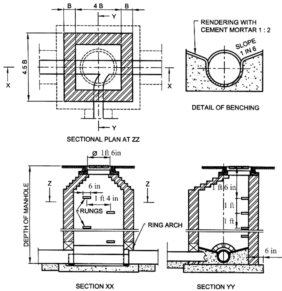
Fig. 5d.14 Detail Of Manhole (Depth Less Than 3 Feet)
