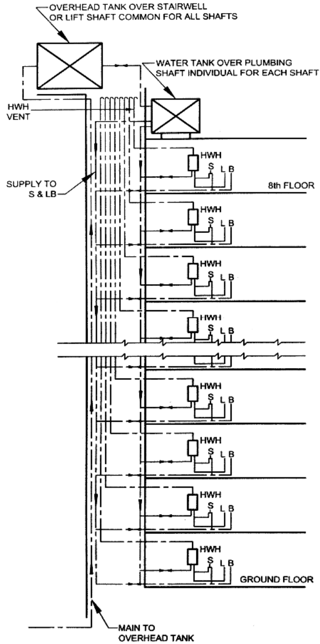
Figure 9 Installation For 8 – Storeyed Building
