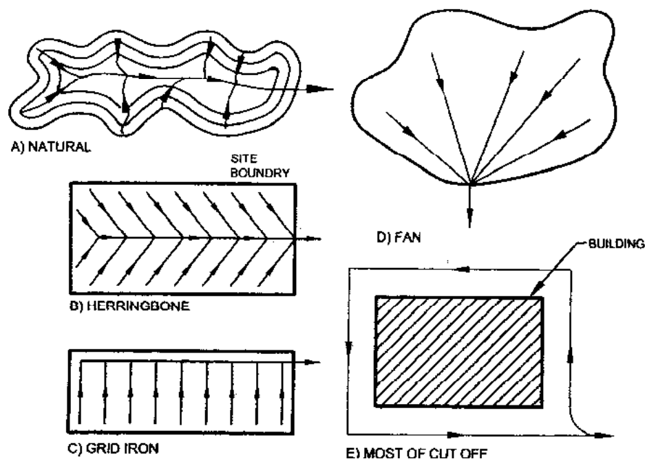
Fig. 19 Details Of Drainage System
