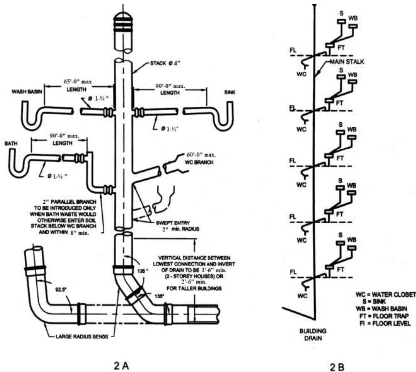
Figure 2 Single Stack System – Main Feature Of Design
