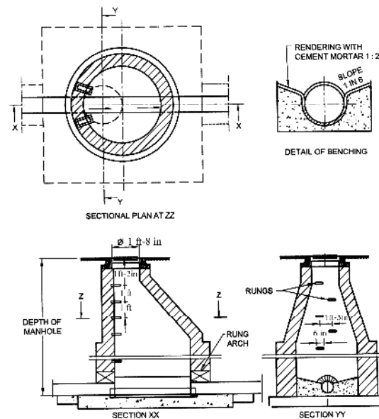
Fig. 5d.16 Detail Of Manhole ( Depth 8 Ft And Above )
