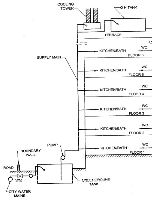
Figure 6 Direct Pumping System Applicable where There is Continuous Demand on System
