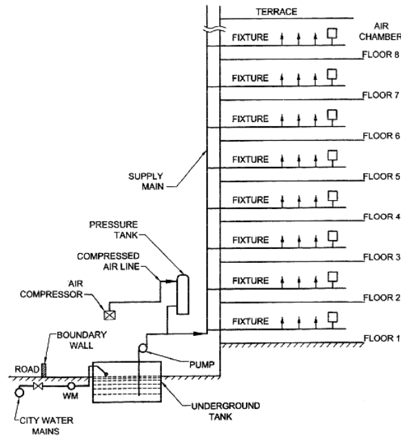
Figure 7 Hydro-Pneumatic System
