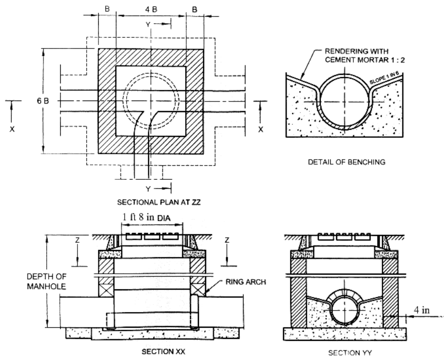
Fig. 5d.15 Detail Of Manhole (Depth 3 Feet And Up To 8 Feet )
