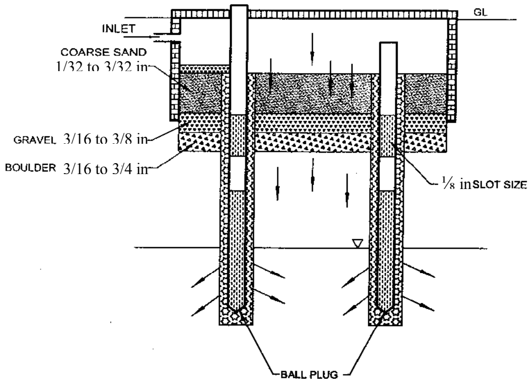
Fig. 5d.18 Artificial Ground Water Recharge Structure
