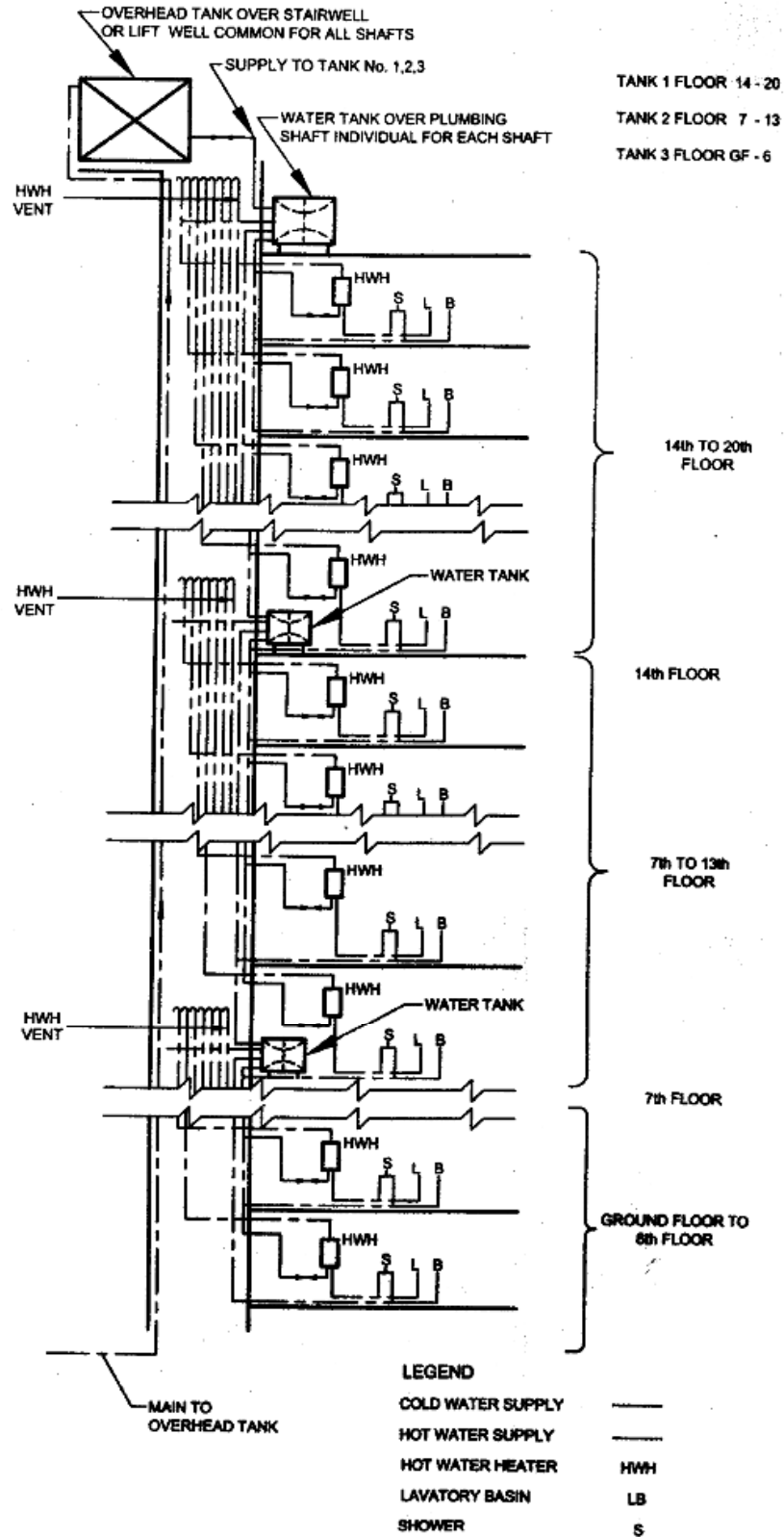
Figure 10 Installation For 20 – Storeyed Building
