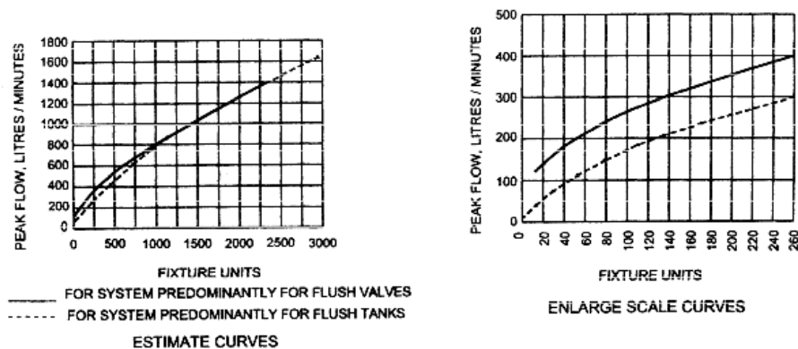
FIG. 5D.13 PEAK FLOW LOAD CURVES
